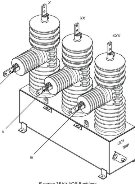
E-series 38 kV ACR Bushings
