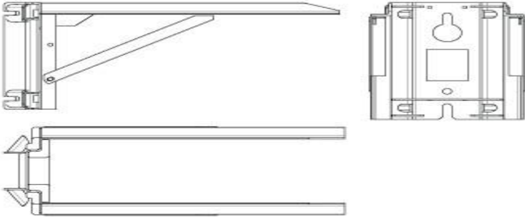
27 kV/38 kV mounting bracket for wooden pole (through holes mounting) (Same mounting bracket for end and center mounting)
