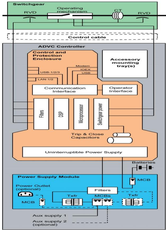
ADVC Controller block diagram
