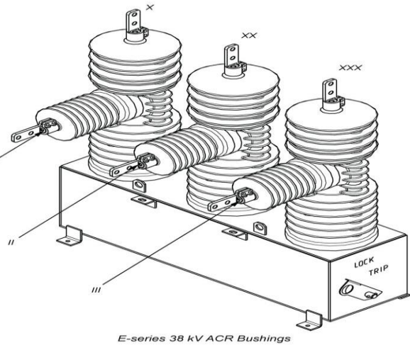
E-series 38 kV ACR Bushings
