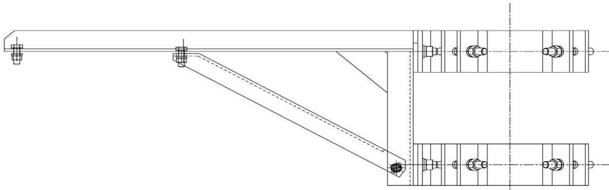
27 kV/38 kV Mounting bracket assembly (Same mounting bracket for end and center mounting)
