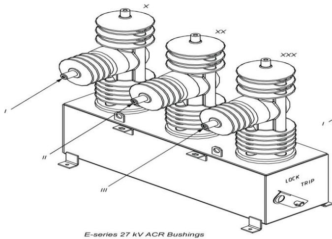
E-series 27 kV ACR Bushings
